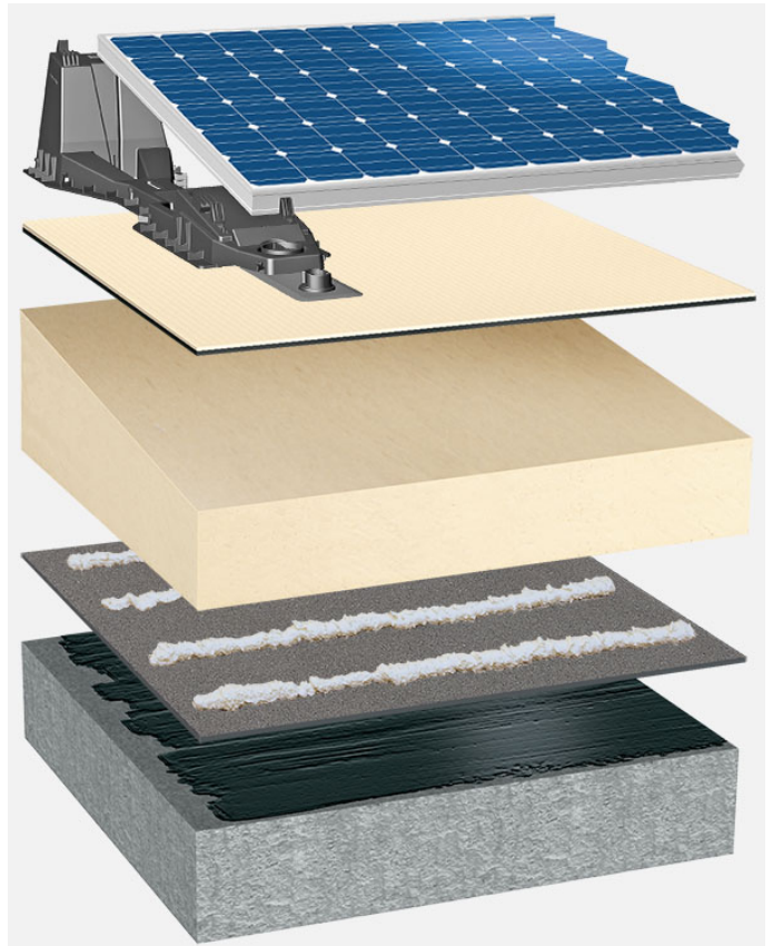
System build-up: BP_PIR-TG_T_01_PVFD
