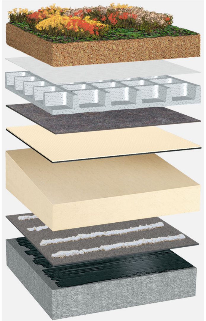
System build-up: BP_PIR-TG_T_01_G75
