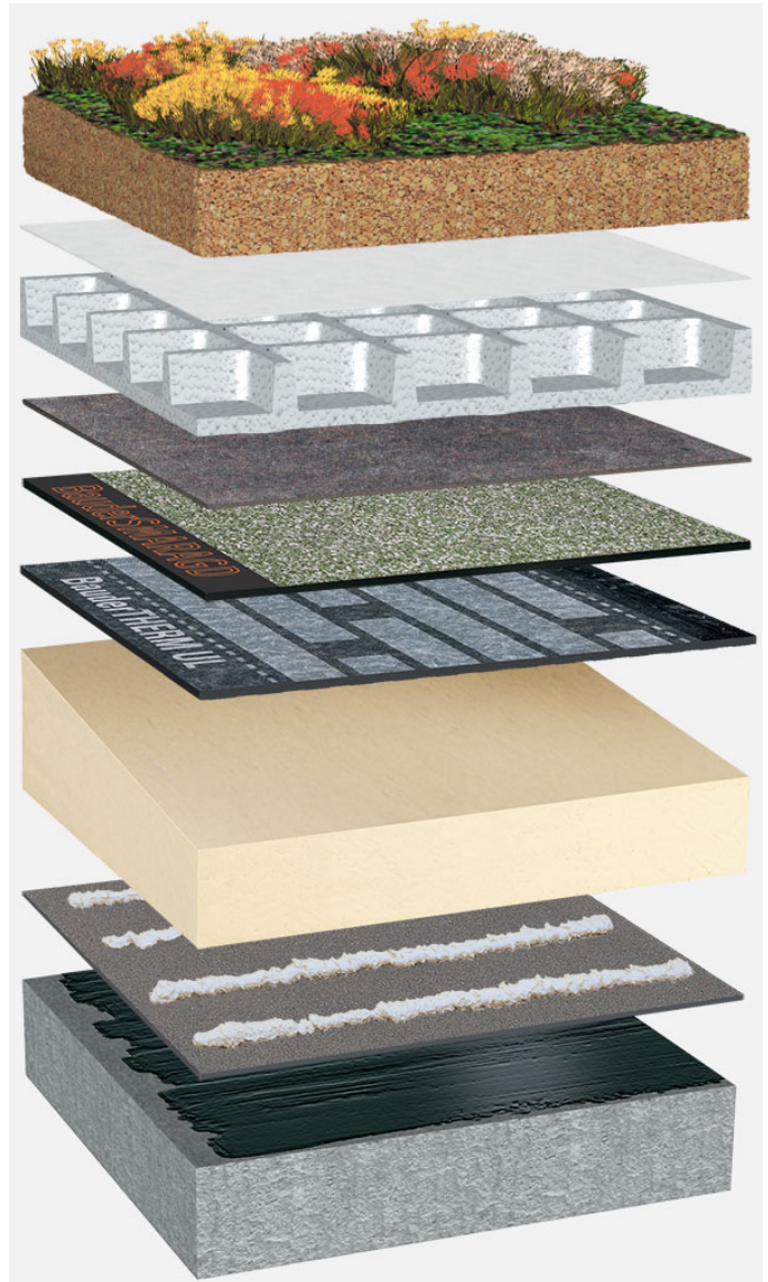
System build-up: BP_PIR-TG_S_01_G75
