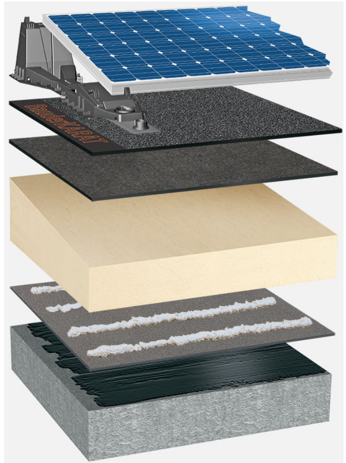
System build-up: BP_PIR-TG_K_01_PVFD
