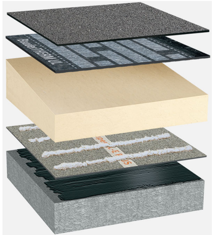
System build-up: BP_PIR-TG_B_01
