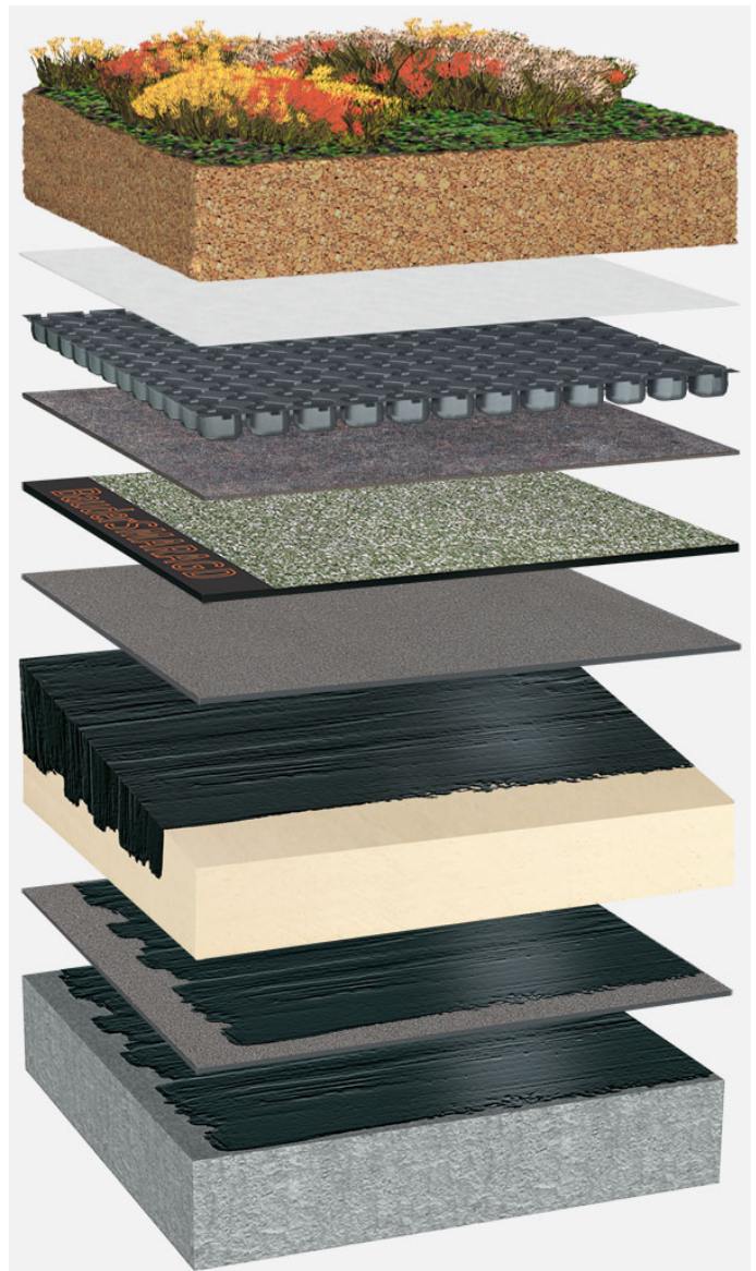
System build-up: BP_PIR-KG_S_01_G125
