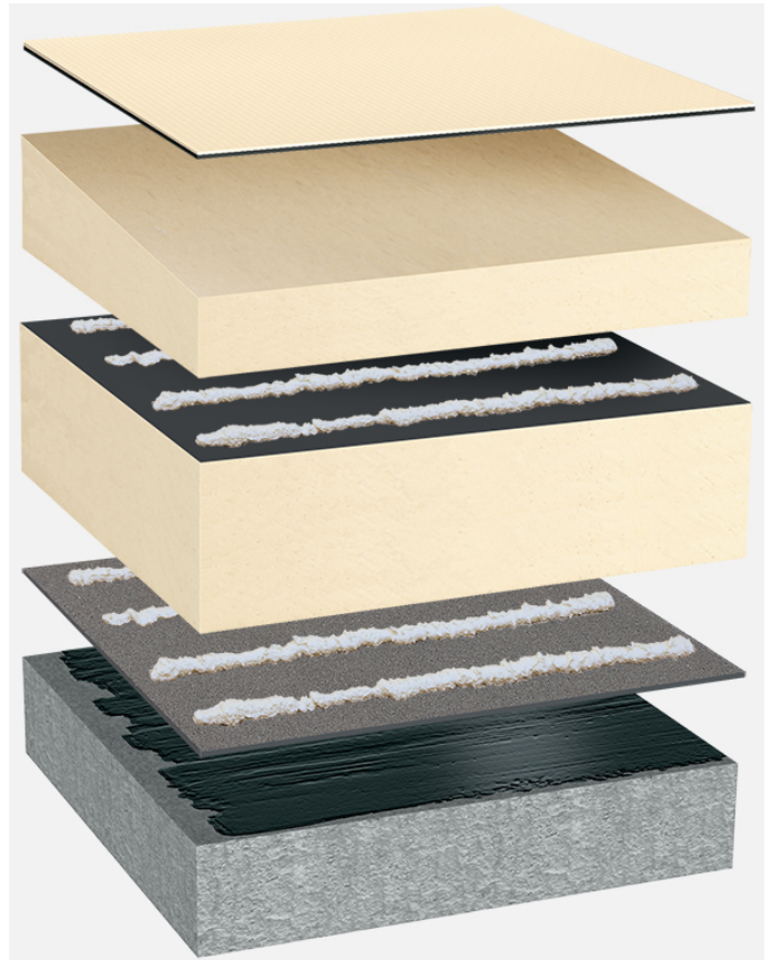
System build-up: BP_PIR-FA_PIR-TG_T_01
