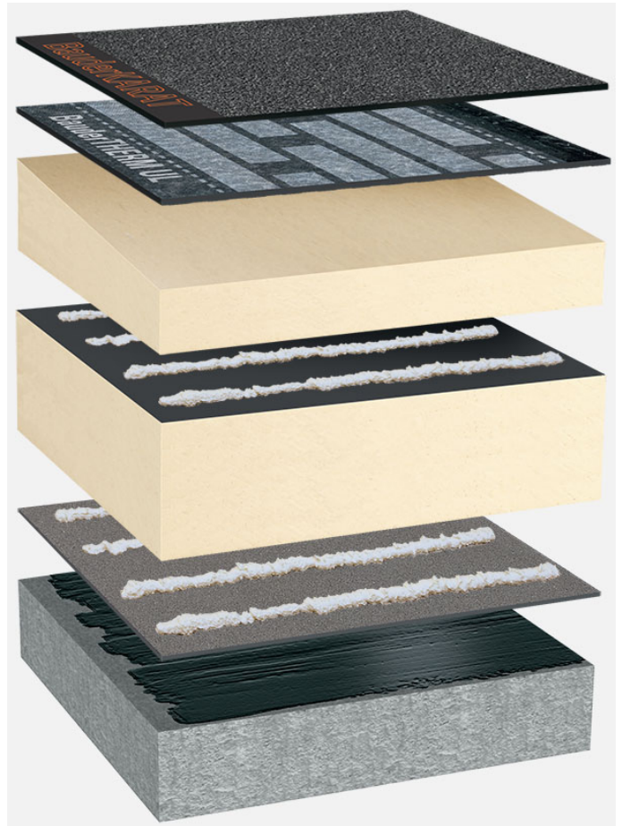
System build-up: BP_PIR-FA_PIR-TG_K_01
