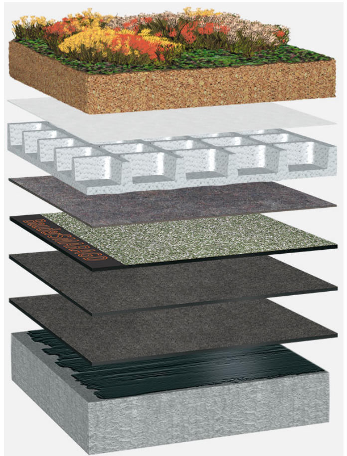
System build-up: BG_S_02_G75
