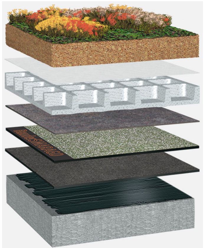
System build-up: BG_S_01_G75
