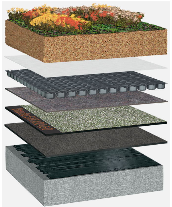
System build-up: BG_S_01_G125
