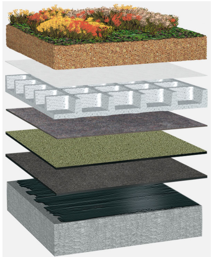
System build-up: BG_P_01_G75
