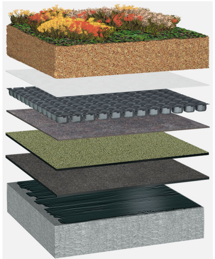
System build-up: BG_P_01_G125
