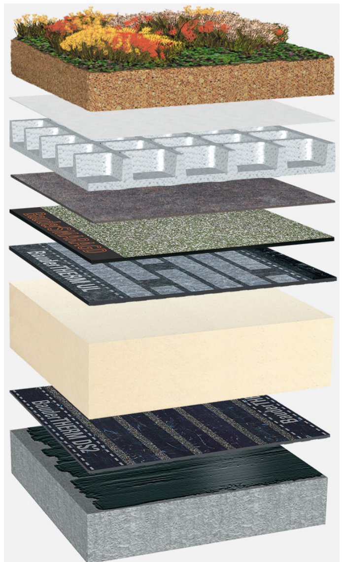
System build-up: BG_PIR-MF_S_01_G75
