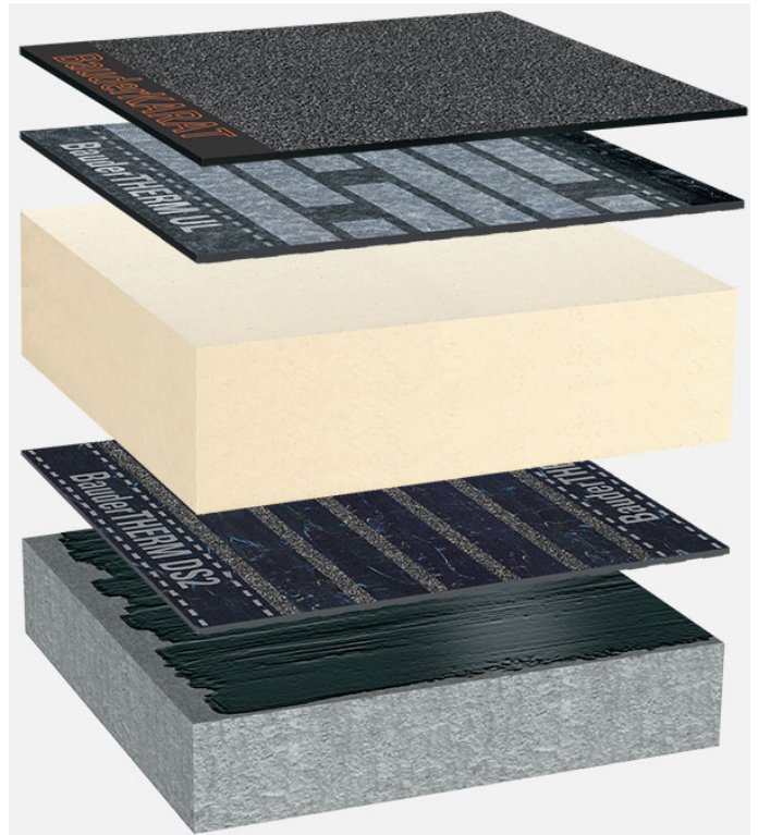
System build-up: BG_PIR-MF_K_01
