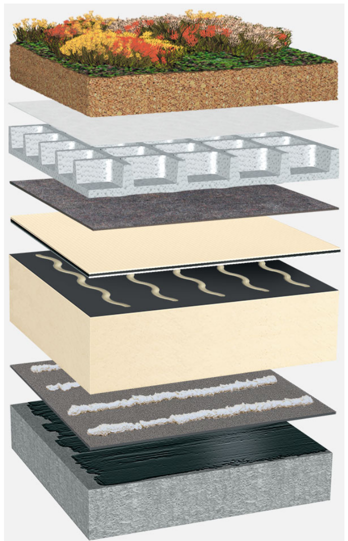
System build-up: BG_PIR-FA_TV_01_G75
