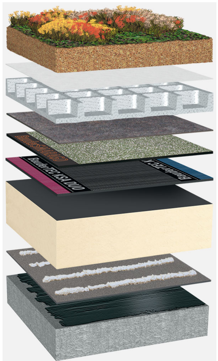
System build-up: BG_PIR-FA_S_01_G75
