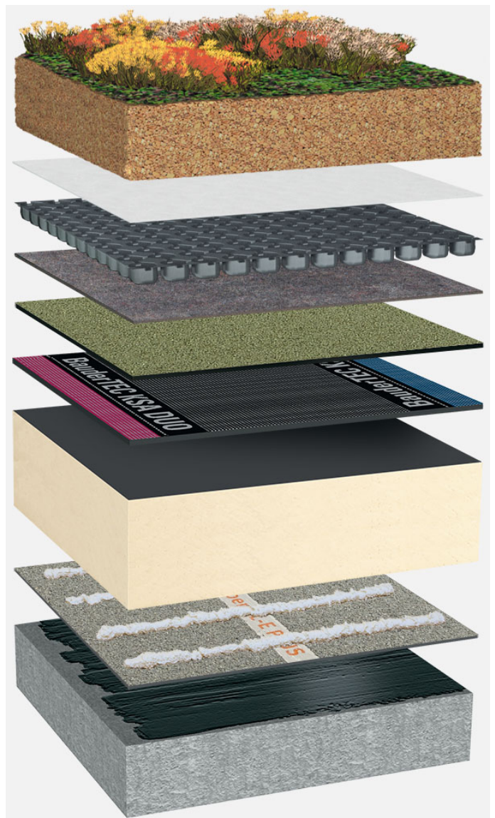
System build-up: BG_PIR-FA_P_01_G125
