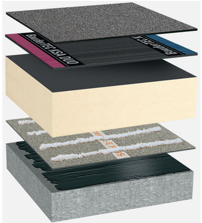
System build-up: BG_PIR-FA_B_01
