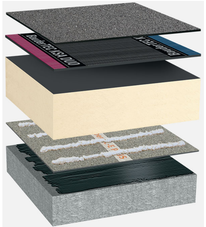
System build-up: BG_PIR-FA_B_01
