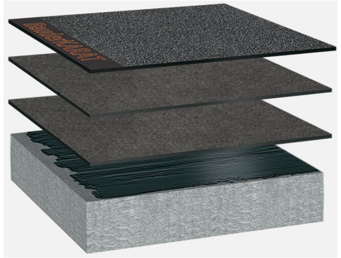
System build-up: BG_K_02
