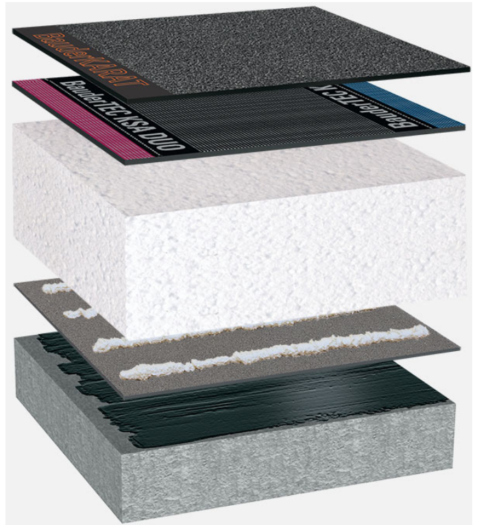
System build-up: BG_EPS-P_K_01
